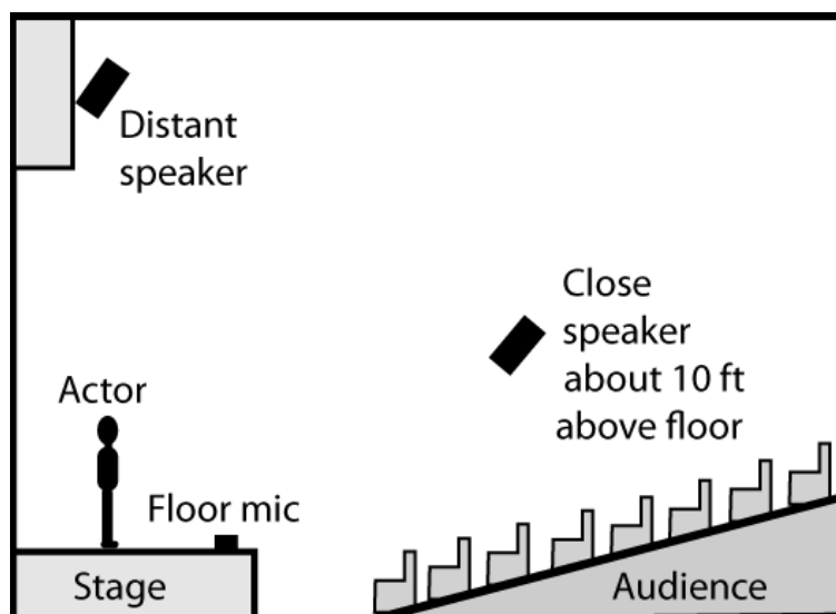
SIDE VIEW OF THEATRE
